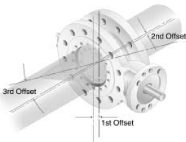
Double Flanged type
